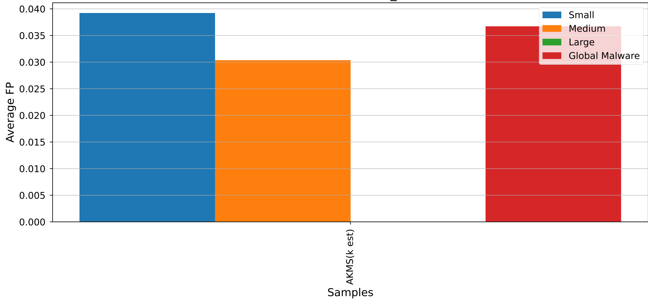
Malicious FP: Cluster2_Size100
